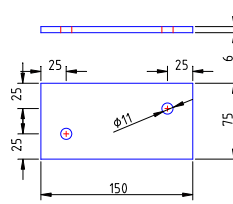
INTERIOR REINFORCING PLATE x 2
