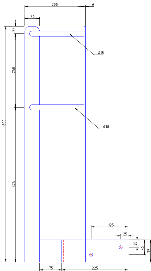
SELLWOOD ROOF HATCH SAFETY HANDRAIL
