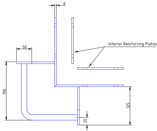
ROOF HATCH SAFETY HANDRAIL (PLAN VIEW)
