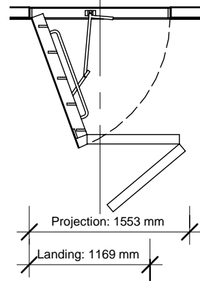
Projection & Landing 1 : 50
