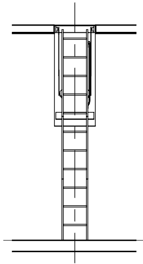
RN28 Front 1 : 50
