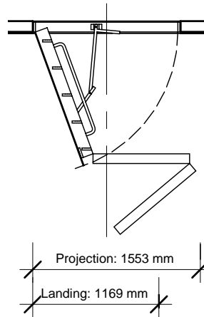
Projection & Landing 1 : 50
