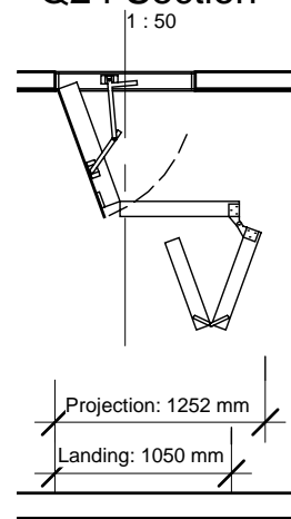
Projection & Landing 1 : 50
